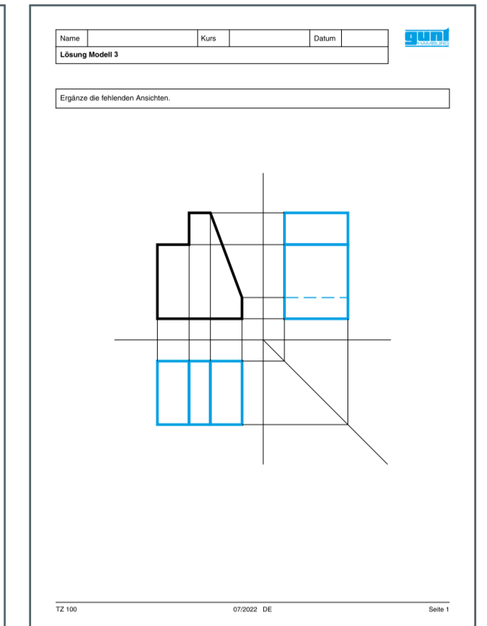
Solution sheet: Drawing the three views with guide lines
