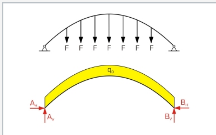
Top: forces on the statically indeterminate parabolic arch, bottom: free-body diagram with line load q_0 in yellow (generated from evenly distributed point loads F ) and bearing reactions F_A + F_B in red
