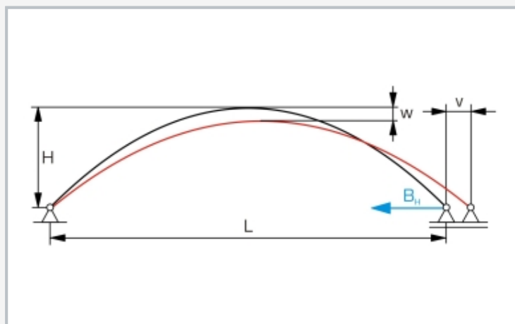
Deformation of the statically determinate arch under line load (red): L length, H height, w deflection, v horizontal displacement on the floating bearing; black arch without load
