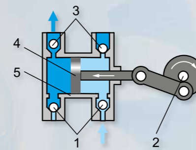
Piston pump
