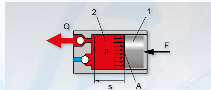
1 displacement body, 2 working chamber; Q flow rate, F displacing force, A area, p delivery pressure, s displacement distance
