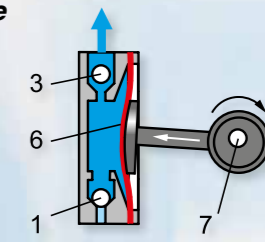
Diaphragm pump
