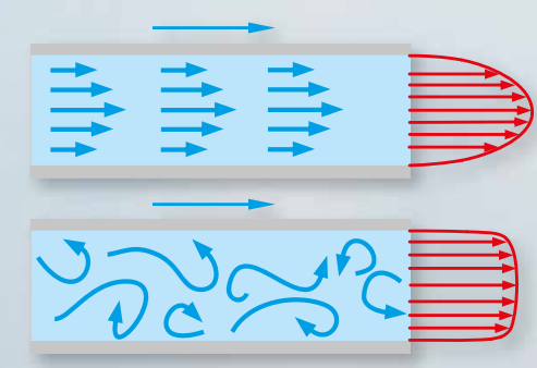
Laminar and turbulent flow profile in pipelines
